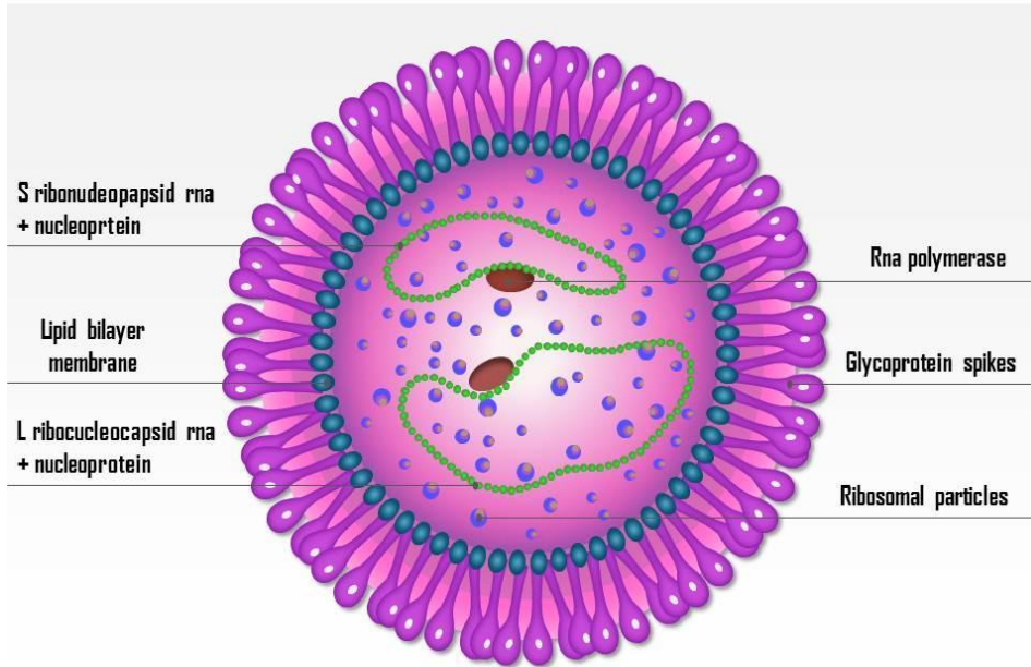
Arena Virus Particle Structure
